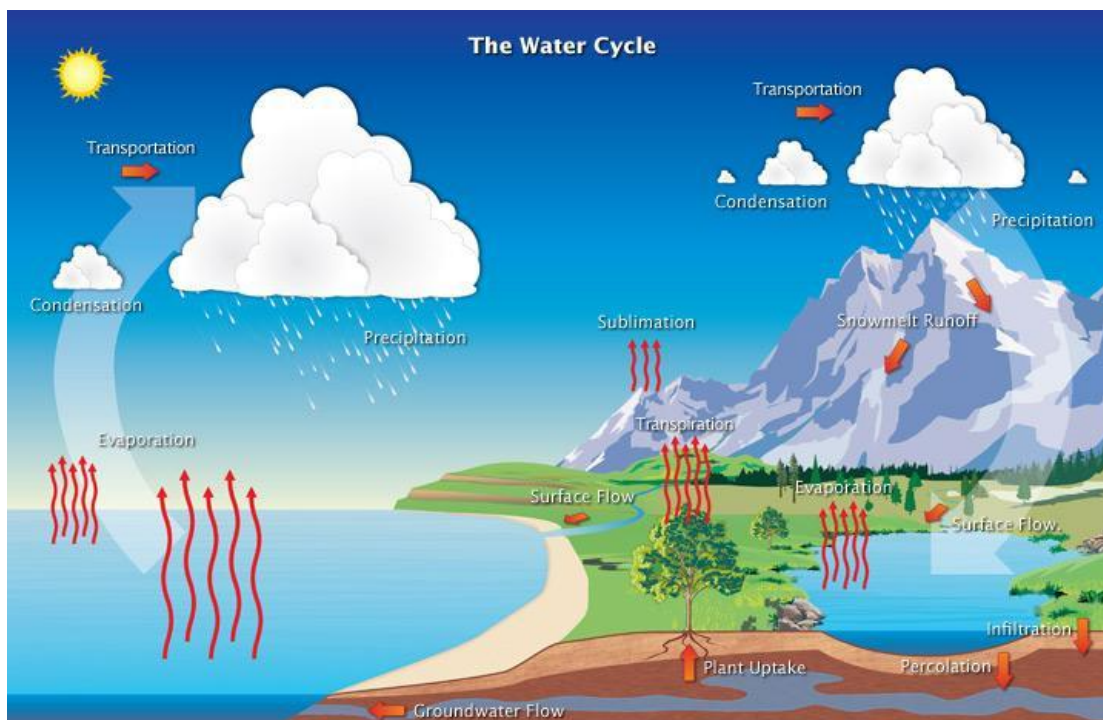
Figure 3.2: Hydrological/Water Cycle
